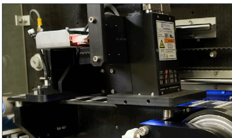
Intelligent automatic UV curing system ensures all printed labels are UV cured even under line stoppages.
